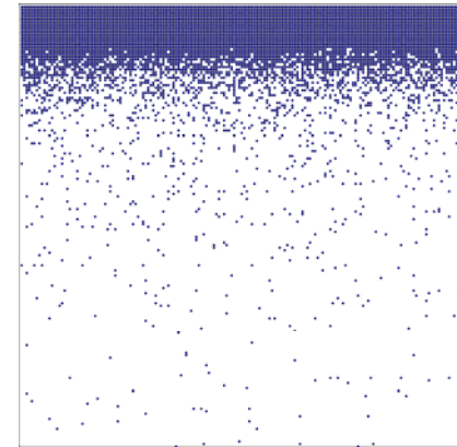
Lower part of the spectrum (GRID'25, 5995 items )
